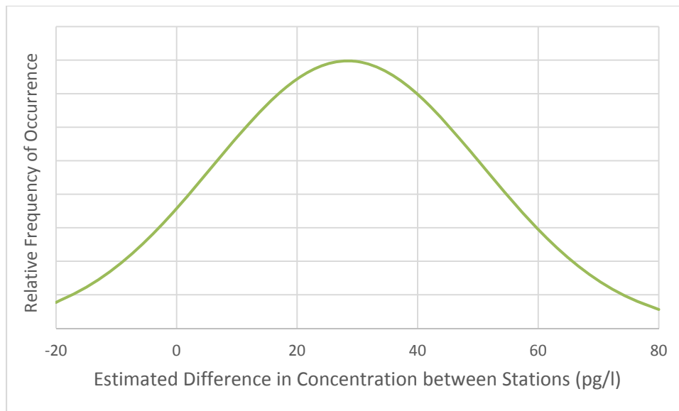
Figure 1. Frequency Distribution for Estimated Difference in Concentration between Stations for the Example where True Upstream Concentration is 72 pg/l and Downstream Concentration is 100 pg/l
