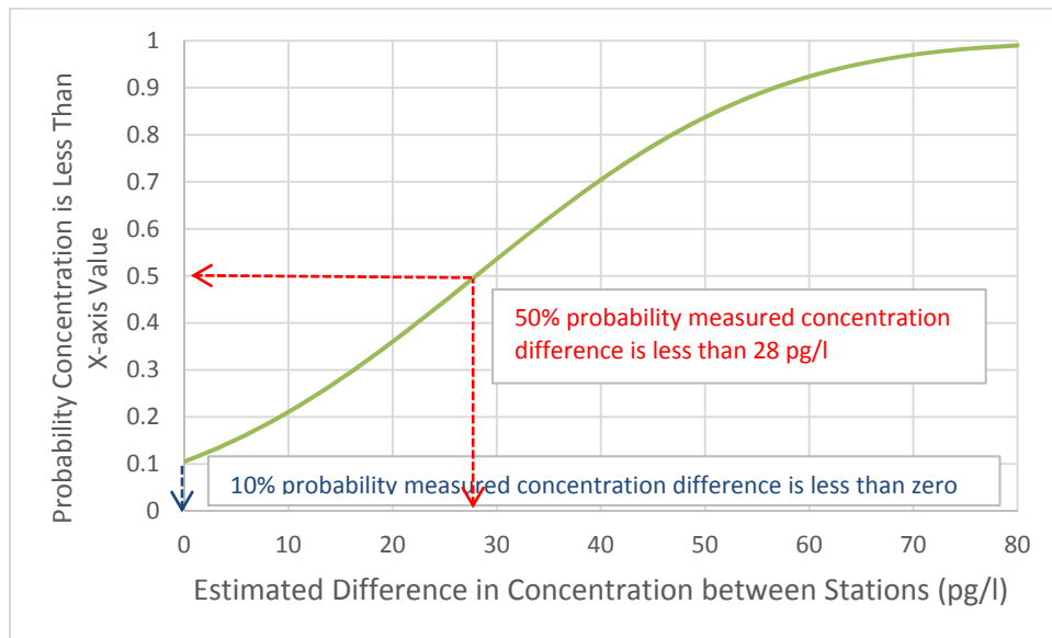
Figure 2. Cumulative Frequency Distribution for Estimated Difference in Concentration between Stations for the Example where True Upstream Concentration is 72 pg/l and Downstream Concentration is 100 pg/l
