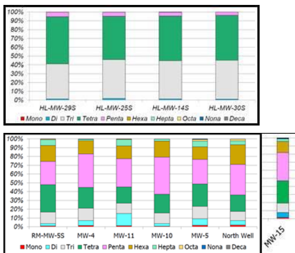
Figure 6. Homolog Distribution of Groundwater Monitoring Data Collected from Kaiser Plume (top) and Up-Gradient/Cross-Gradient Wells (bottom)
