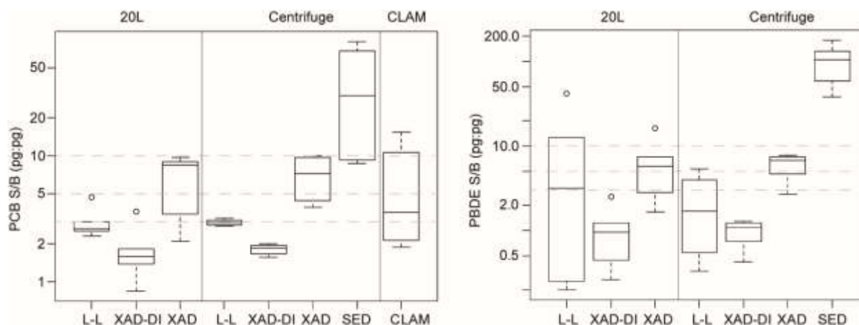
Figure 11: The range in sample:blank (S/B) of PCB (left) and PBDE (right) concentrations for all sampling approaches.
