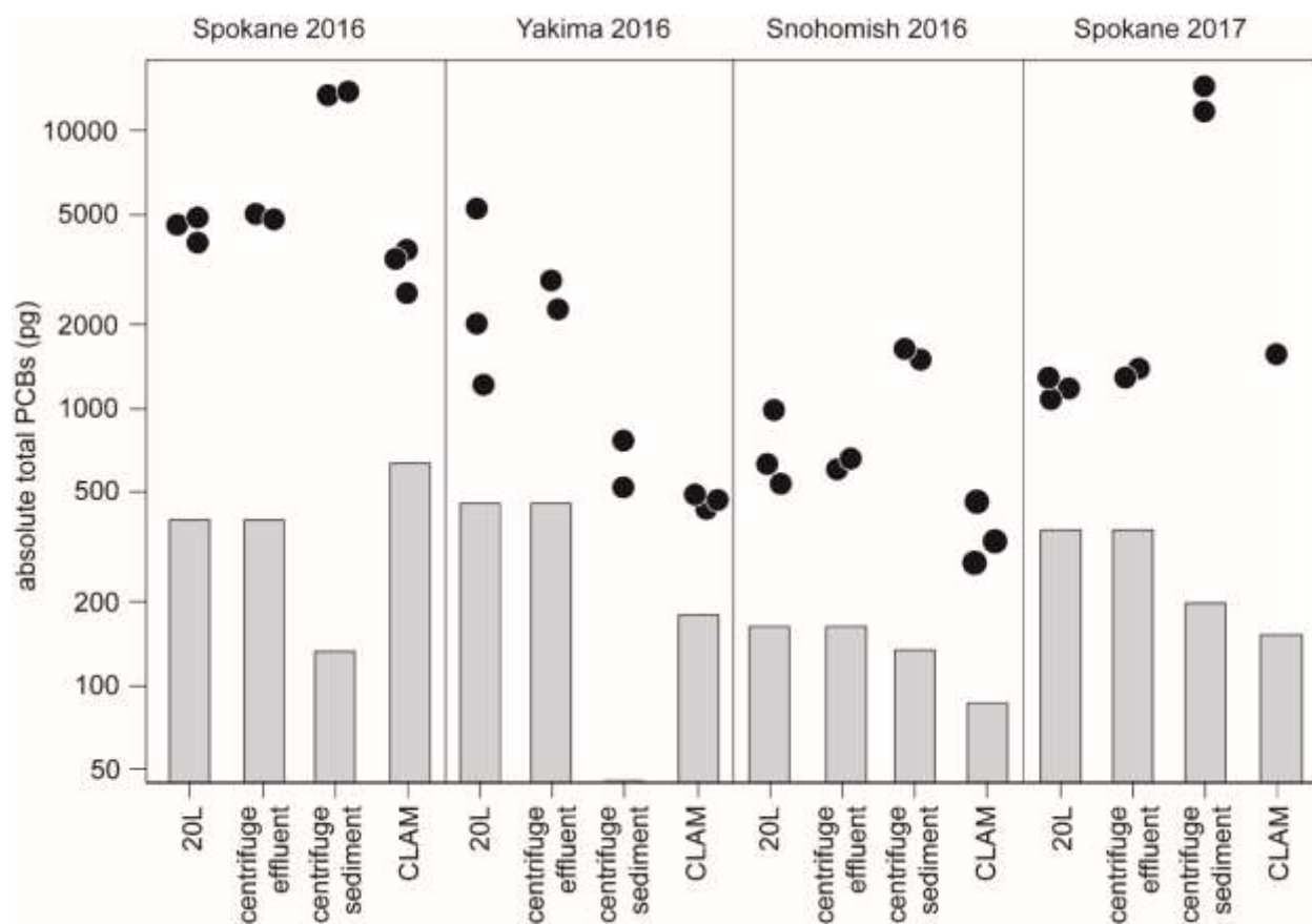
Figure 7: Absolute PCB mass in the blank (grey bars) and environmental (black dots) samples.
