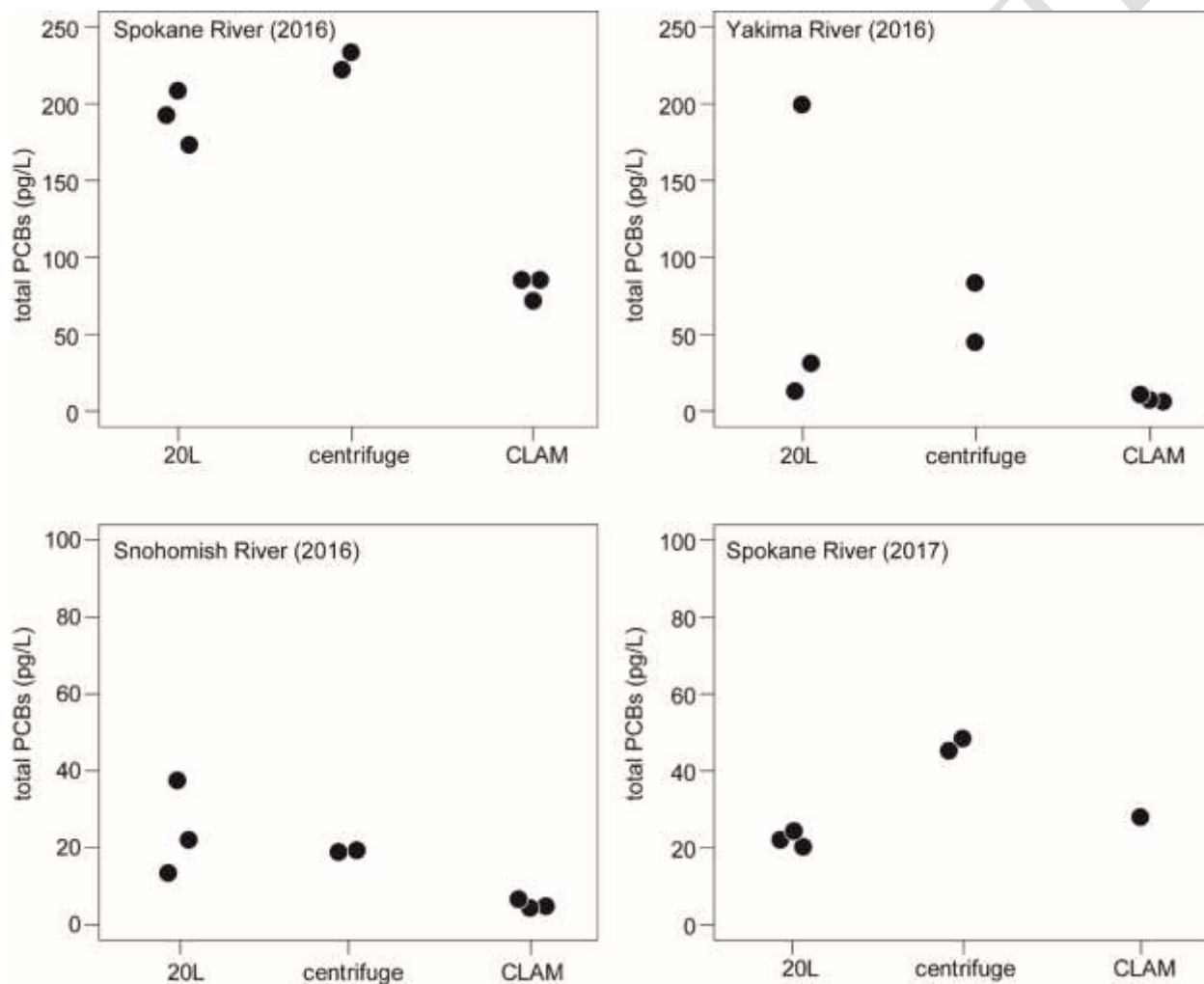
Figure 8: Blank-censored total PCB results for each sampling event.
