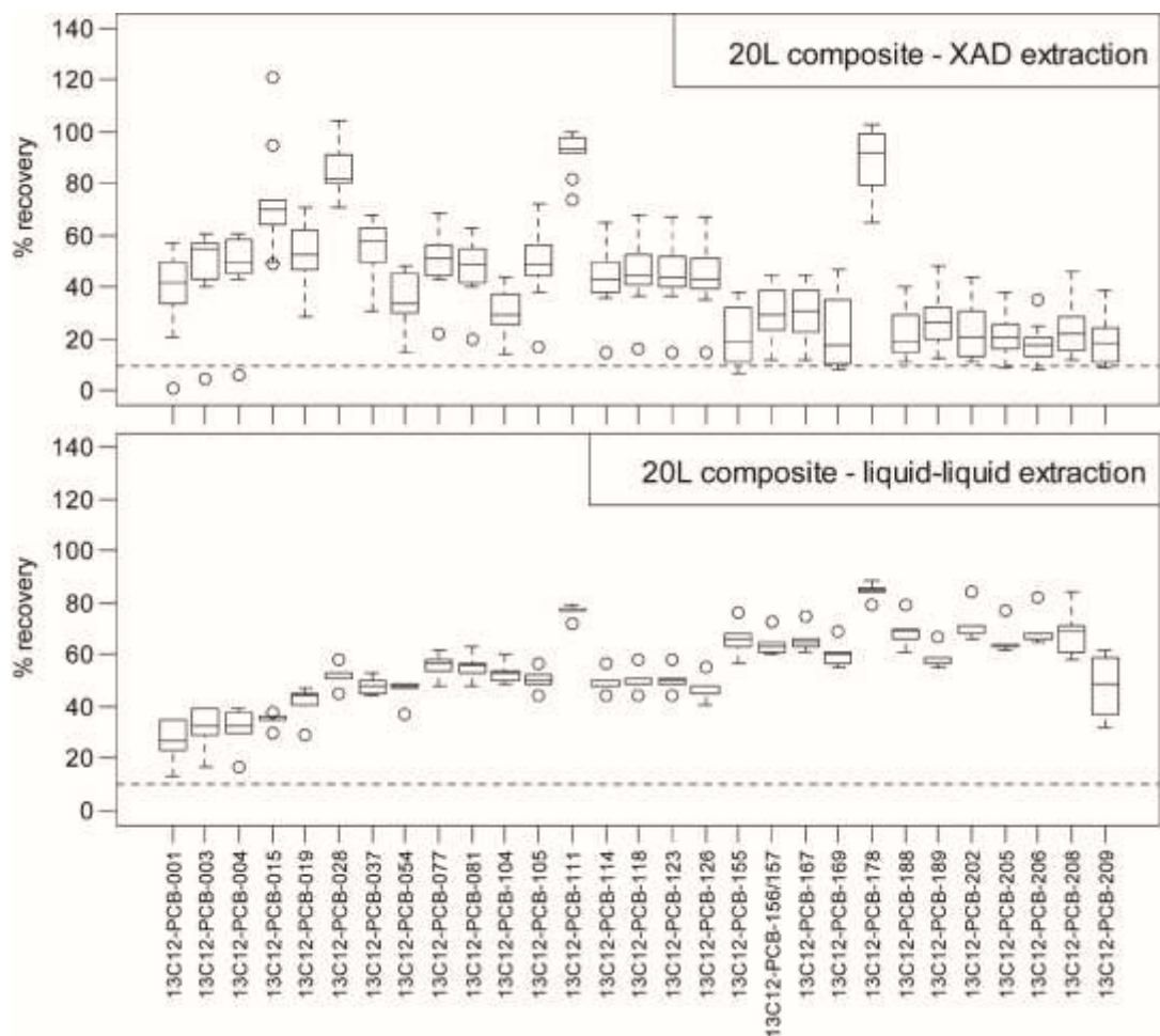
Figure C-2: Box and whiskers plot of the recoveries for the isotopically-labeled PCB congeners between large volume extraction techniques.
