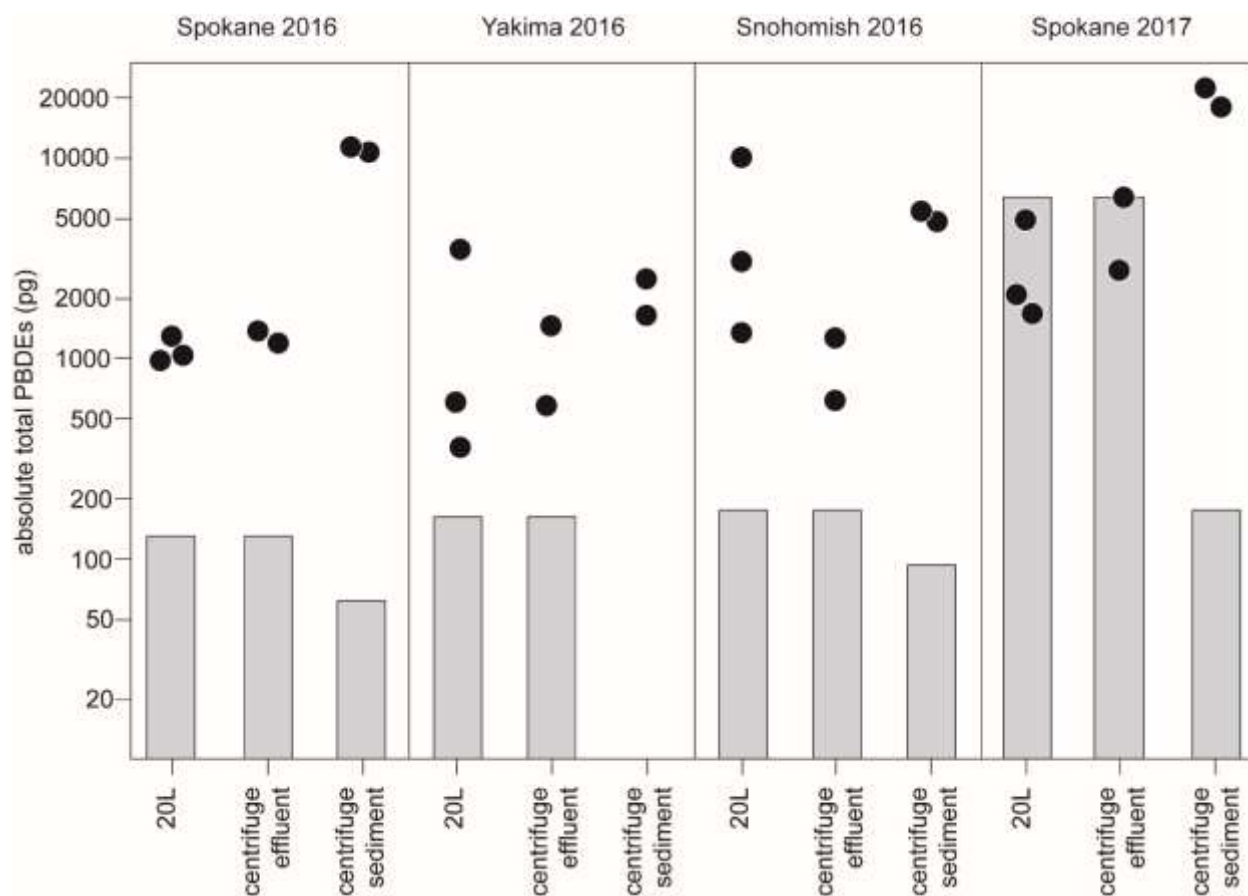
Figure 9: Absolute PBDE mass in the blank (grey bars) and environmental (black dots) samples.
