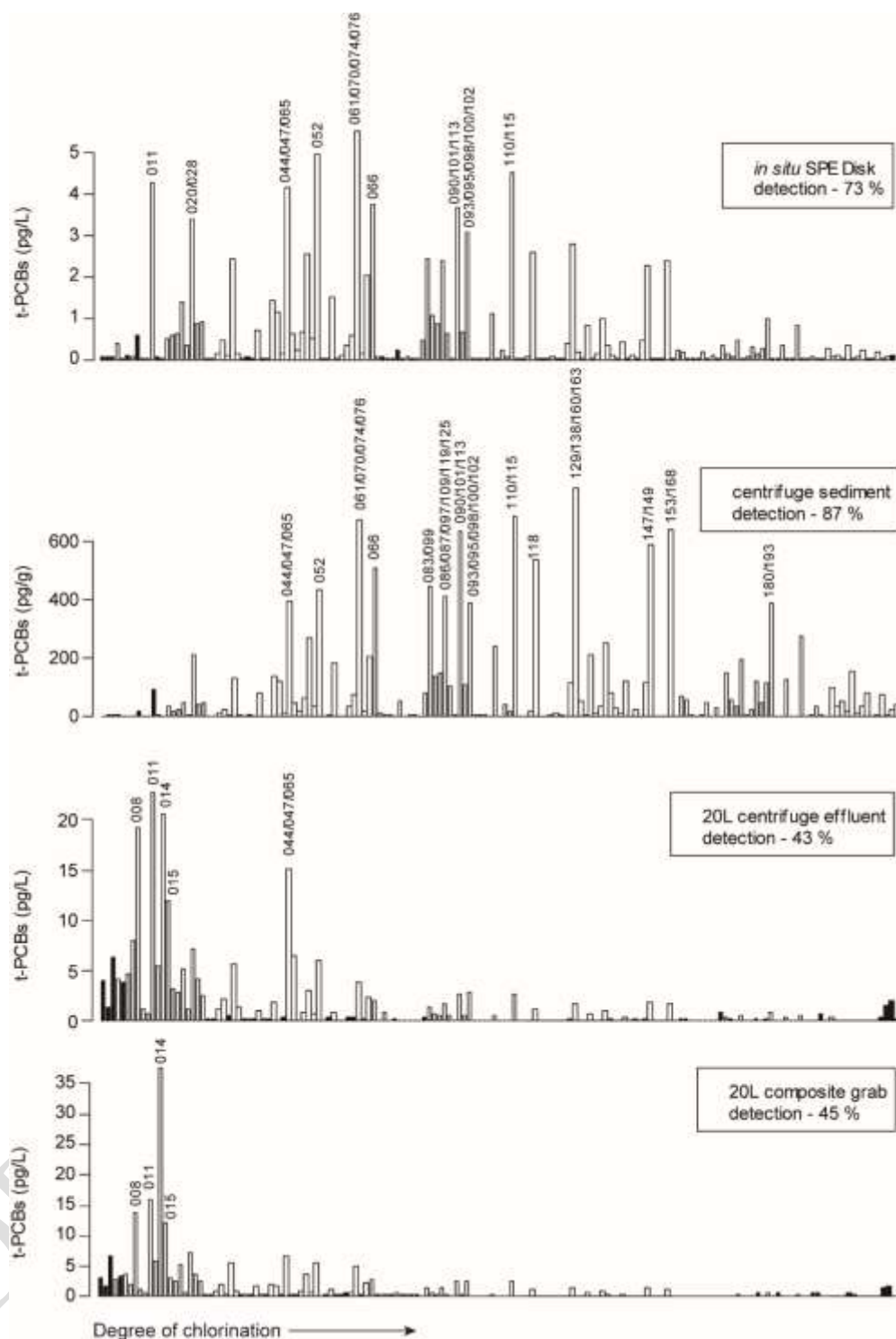
Figure 14: PCB congener profiles among the different sampling approaches from the Spokane River.
