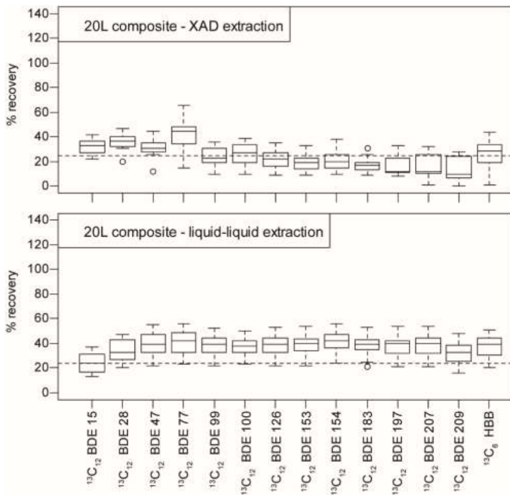
Figure D-2: Box and whiskers plot of the recoveries for the isotopically-labeled PBDE congeners between large volume extraction techniques.
