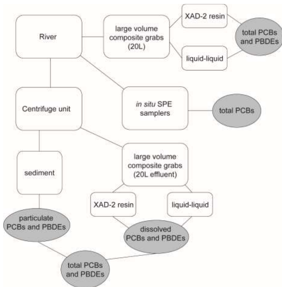
Figure 4: Flow chart of the three sampling approaches and contaminants analyzed.
