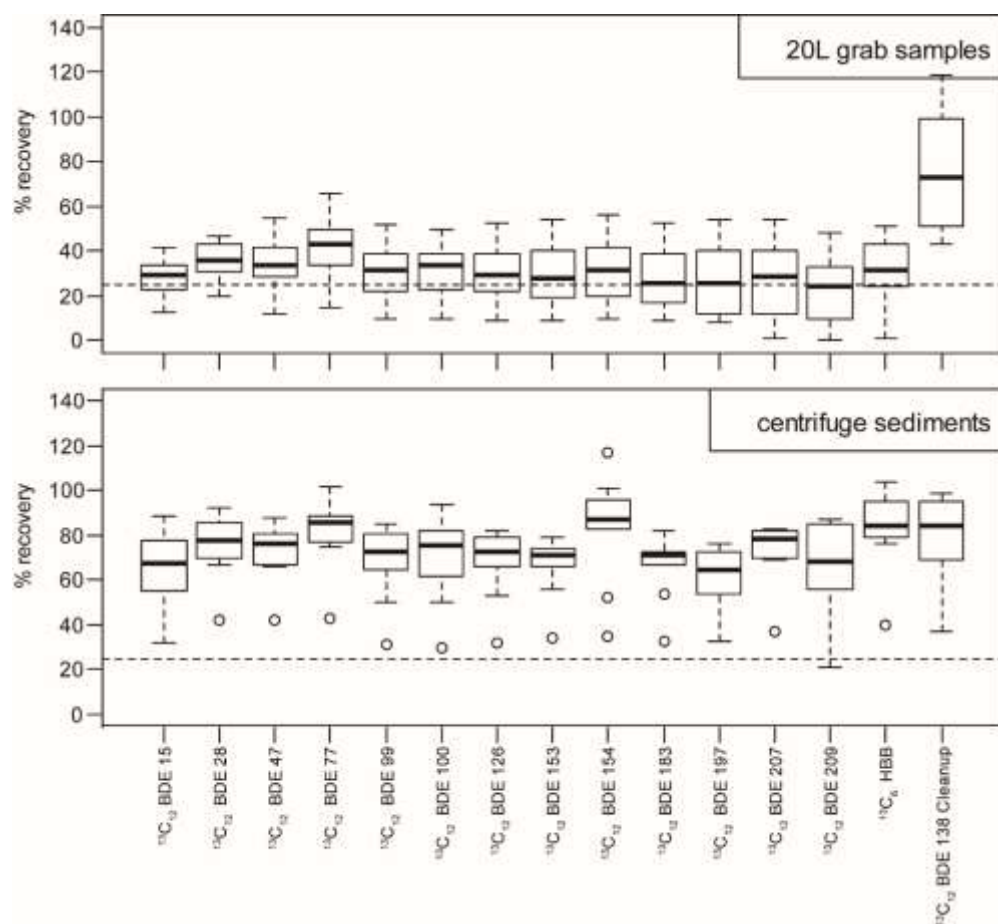
Figure D-1: Box and whiskers plot of the recoveries for the isotopically-labeled PBDE congeners between sampling approaches.
