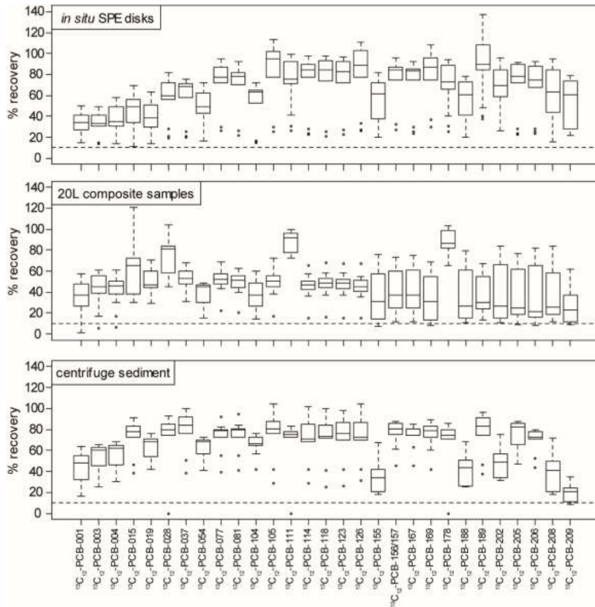
Figure C-1: Box and whiskers plot of the recoveries for the isotopically-labeled PCB congeners among sampling approaches.
