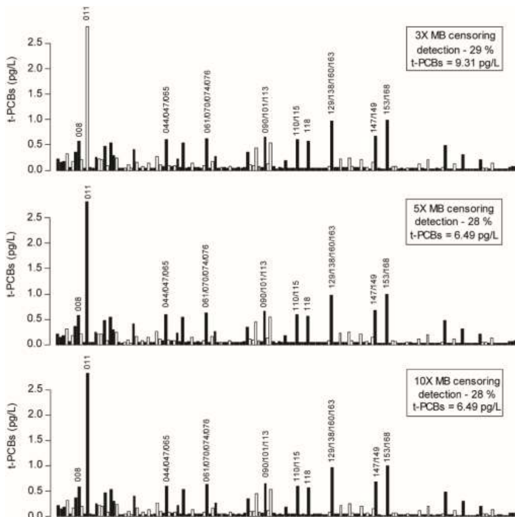
Figure 12: PCB congener profiles from an in situ SPE disk in the Snohomish River under different blank censoring thresholds.
