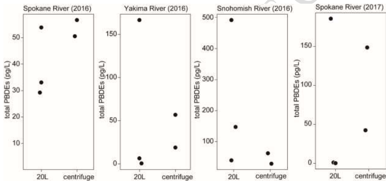
Figure 10: Blank-censored total PBDE results for each sampling event.
