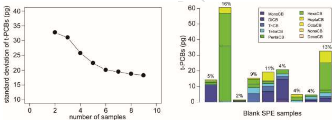
Figure 13: Standard deviation among SPE blanks (left) and PCB homologue distributions in the blanks (right).
