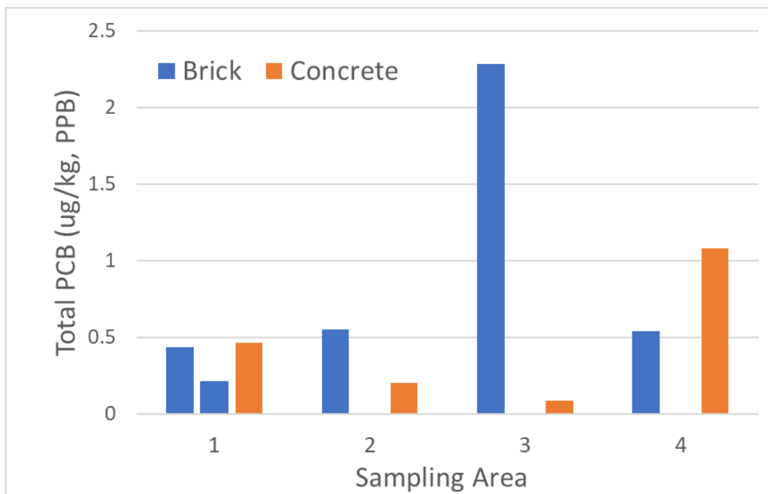
Figure 2. Spokane River Artificial Fill Total PCB Concentrations ( \mu\text{g}/\text{kg} )
