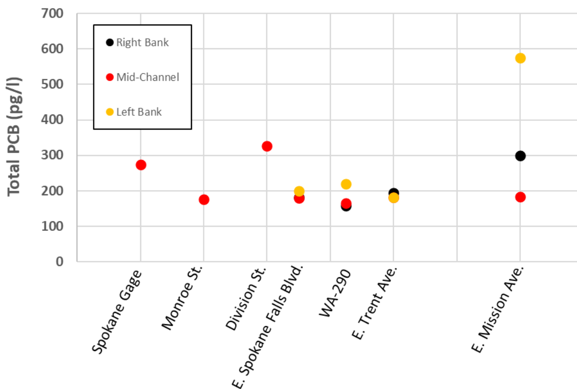
Figure 2. Water Column Total PCB Concentrations (pg/l)
